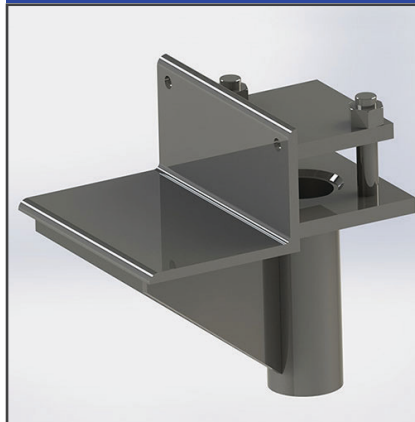
Standard Underpinning Lift Bracket
